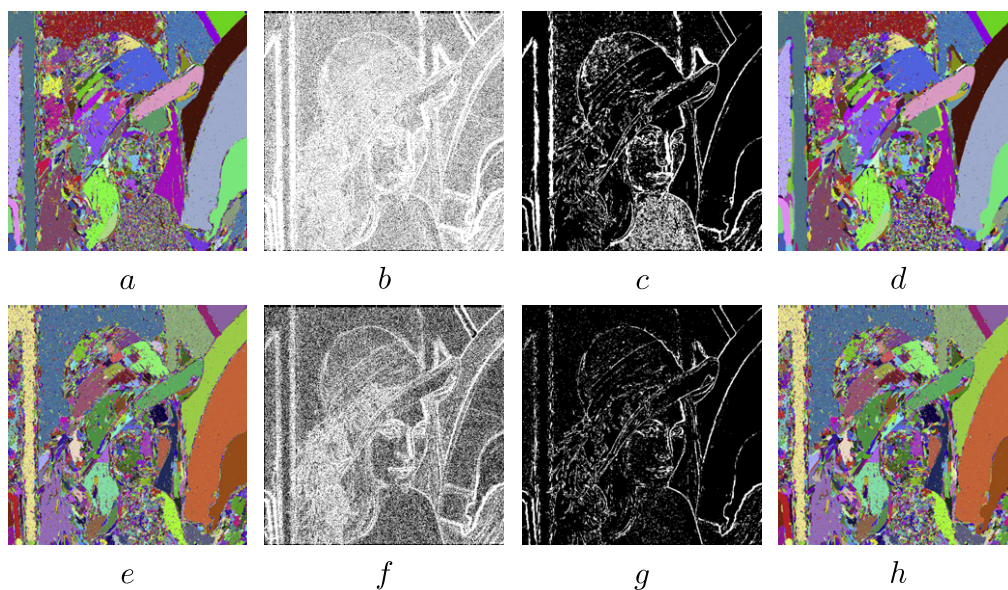
Fig. 4. Transition region filtering: (top) grayscale, (a) C^{x,\omega} using \alpha = \omega = 100 (31,385 QFZ), (b) Transition pixels mask (82% of the image), (c) Transition region mask (19,073 transition regions representing 17% of the image), (d) QFZ after filtering (12,313 QFZ); (bottom) color, (e) C^{x,\omega} using \alpha = \omega = 100 (34,651 QFZ), (f) Transition pixels mask (57% of the image), (g) Transition region mask (12,743 transition regions representing 9% of the image), (h) QFZ after filtering (21,909 QFZ).
