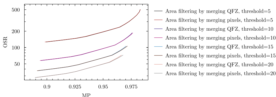
Fig. 12. Comparison between filling removed QFZ using an SRG over QFZ and over pixels, using the proposed filtering approach with C^{(\alpha,\omega)} on Berkeley Segmentation Dataset with different values of minimal area threshold.
