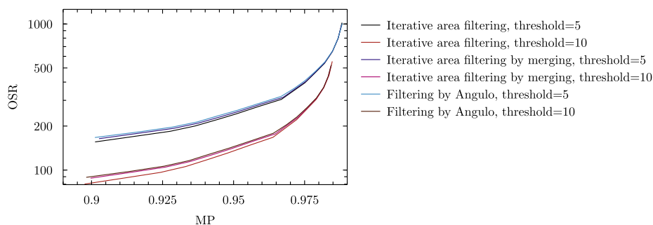
Fig. 16. Comparison of the iterative version of our approach, iterative area filtering and Angulo's approach with C^{\alpha,\omega} on the Berkeley Dataset.
