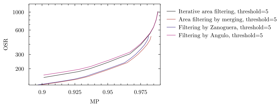
Fig. 14. Comparison of our approach (area filtering by merging) and existing filtering methods based on an area threshold using C^{z,\omega} on the Berkeley Dataset.
