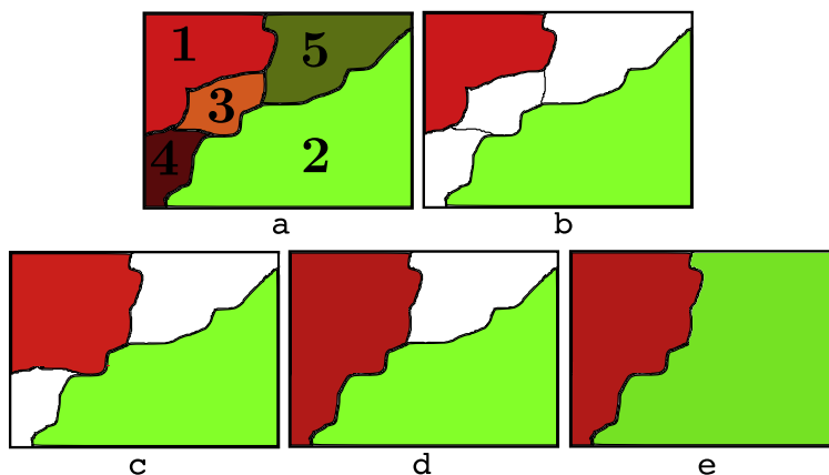
Fig. 10. QFZ area filtering by merging: (a) original QFZ, (b) Removal of QFZ which area is less to the area threshold, (c) first SRG iteration: QFZ 1 \supset QFZ 3, (d) second SRG iteration: QFZ 1 \supset QFZ 4, (e) last SRG iteration: QFZ 2 \supset QFZ 5.
