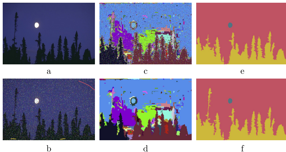
Fig. 20. QFZ-based image segmentation on a noisy image: (a) Original image, (b) Noisy image ( salt & pepper on 10% of pixels) with markers provided by the user, (c) Unfiltered QFZ ( \alpha = \omega = 50 ), (d) Filtered QFZ (area threshold = 20), (e) Segmentation result using unfiltered QFZ, (f) Segmentation result using filtered QFZ.
