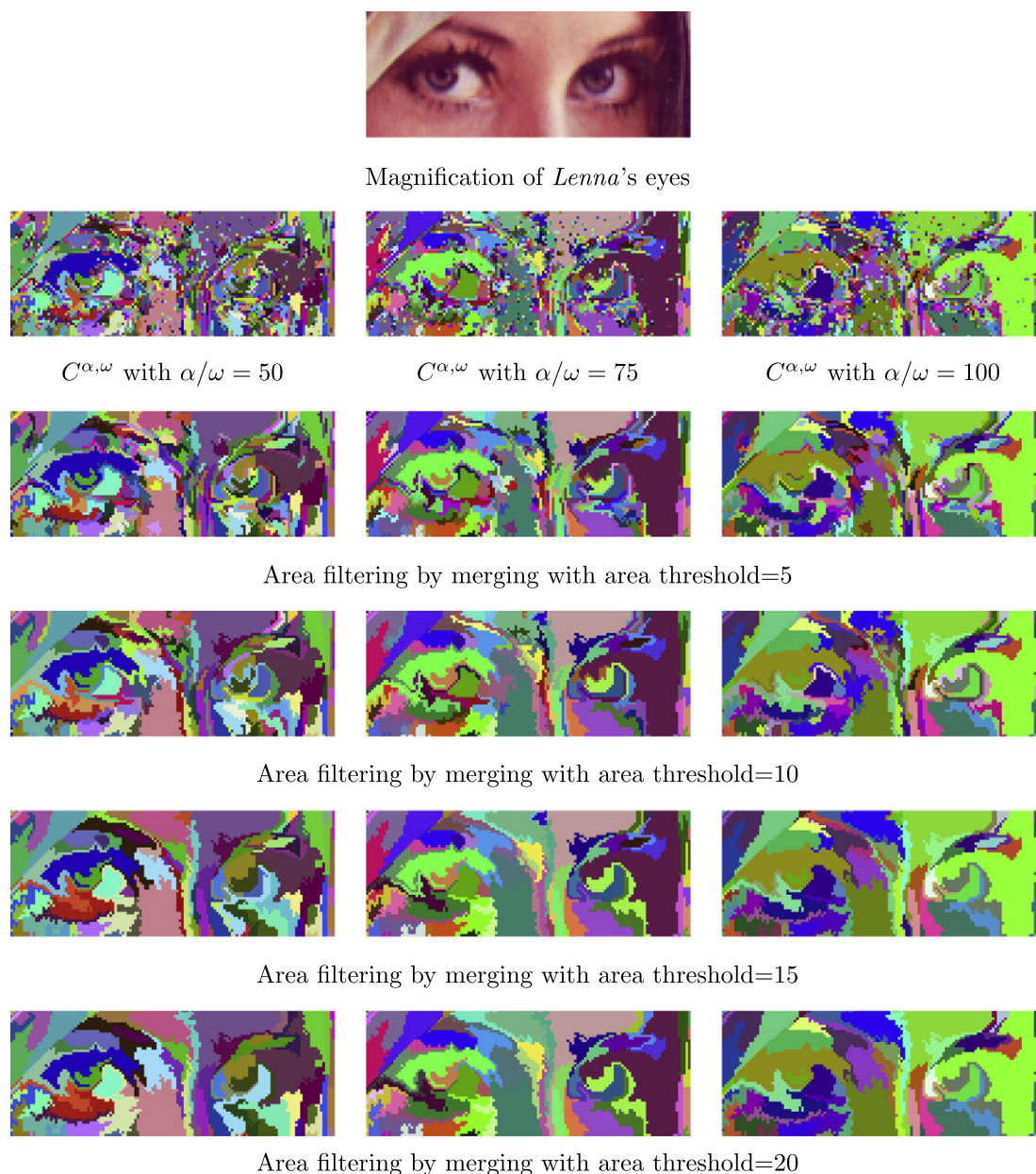
Fig. 13. Illustration of detail conservation with the example of Lenna's eyes and different area threshold and \alpha/\omega values.
