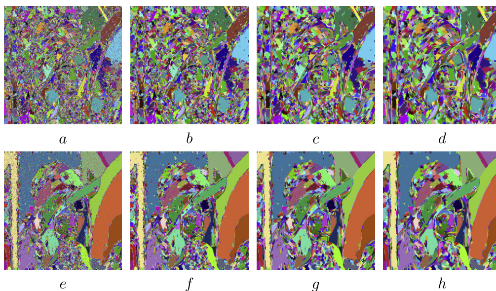
Fig. 11. QFZ area filtering by merging on C^{(\alpha,\omega)} : (top) \alpha = \omega = 50 ; (a) original QFZ (58,219 QFZ); (b) area threshold = 5 (8,014 QFZ); (c) area threshold = 10 (3,572 QFZ); (d) area threshold = 15 (2,219 QFZ); (bottom) \alpha = \omega = 100 ; (e) original QFZ (3,4651 QFZ); (f) area threshold = 5 (4,600 QFZ); (g) area threshold = 10 (2,051 QFZ); (h) area threshold = 15 (1,252 QFZ).
