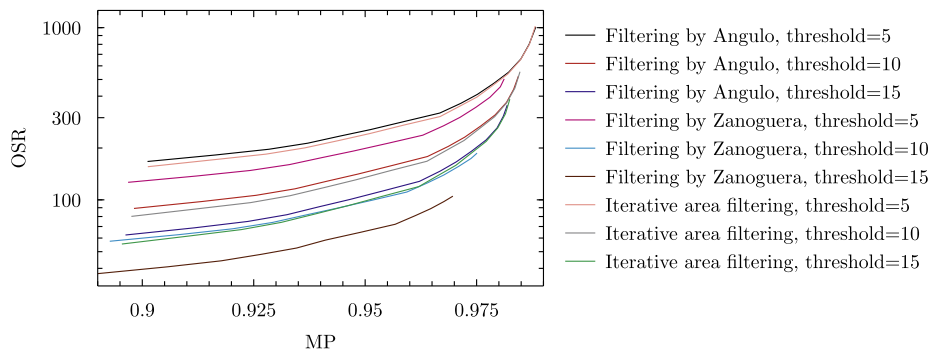
Fig. 9. Filtering approaches based on minimal area threshold comparison using C^{(z,\omega)} on Berkeley Segmentation Dataset with different values of minimal area threshold.
