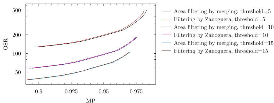
Fig. 17. Comparison of our approach and Zanoguera's approach with C^{\alpha,\omega} on the Berkeley Dataset.
