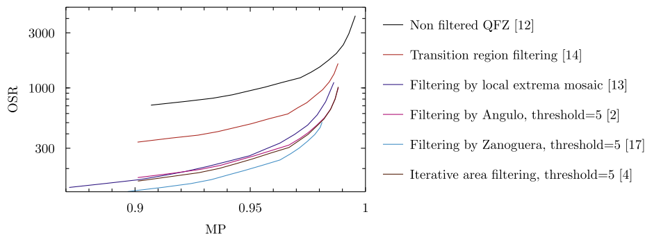
Fig. 8. Existing QFZ filtering approaches comparison using C^{(z,\omega)} on Berkeley Segmentation Dataset.
