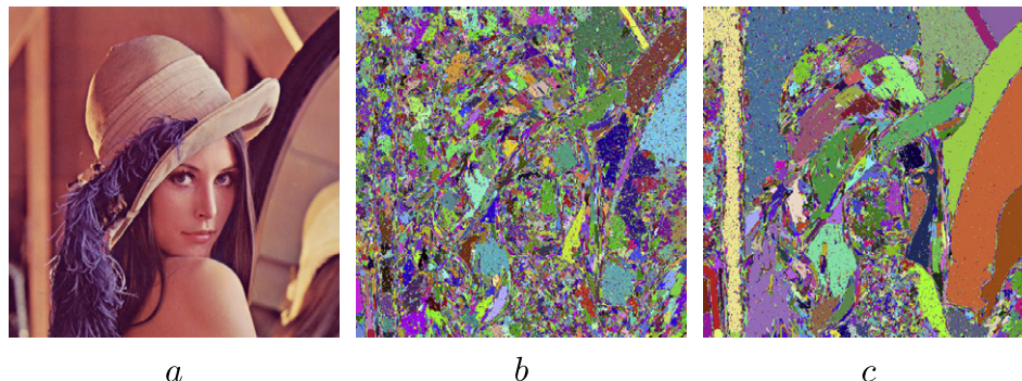
Fig. 2. Oversegmentation on lenna: (a) Original image, (b) C^{\alpha, \omega} using \alpha = \omega = 50 (58,219 QFZ), (c) C^{\alpha, \omega} using \alpha = \omega = 100 (34,651 QFZ).
