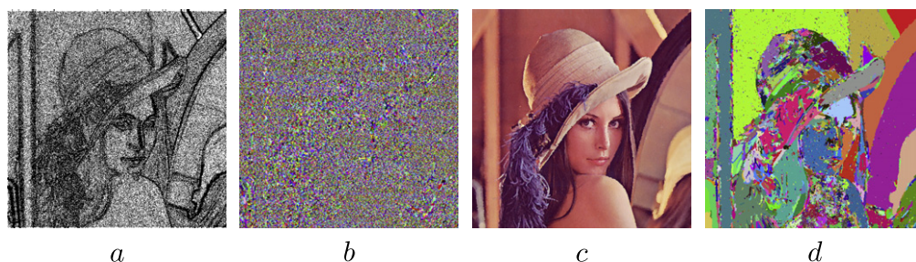
Fig. 5. Filtering by local extrema mosaic: (a) local extrema mask (43% of the image), (b) local extrema mosaic (112,461 regions), (c) original image with reinforced contrast, (d) C^{z,\omega} using \alpha = \omega = 100 on reinforced contrast image (8,045 regions).
