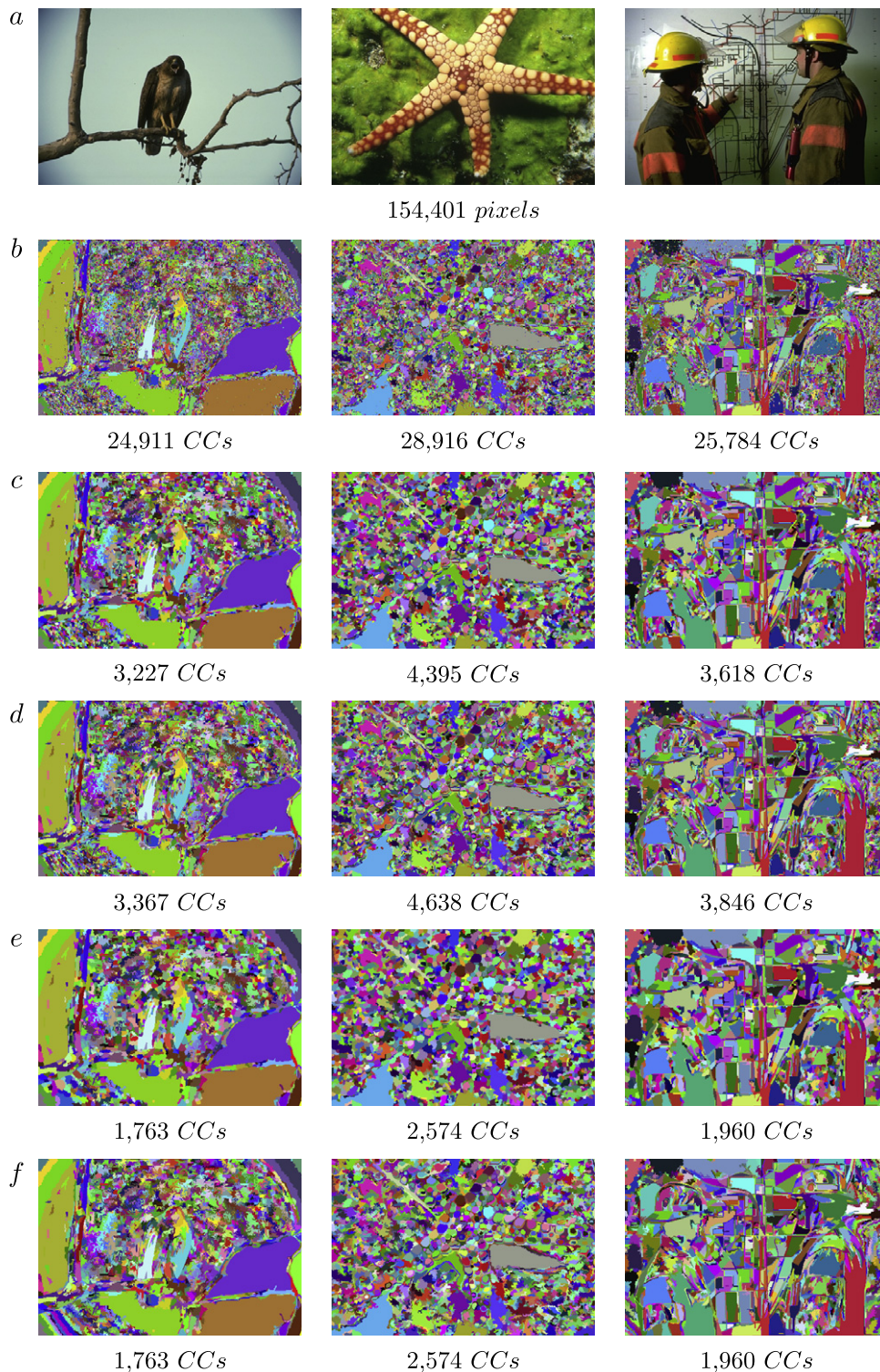
Fig. 15. Visual illustration of results obtained by parametric approaches using C^{x,\omega} on the Berkeley Dataset with \alpha/\omega = 50 and an area threshold = 10. (a) original image; (b) unfiltered QFZ; (c) iterative area filtering; (d) Angulo's approach; (e) Zanoguera's approach, (f) area filtering by merging (proposed approach).
